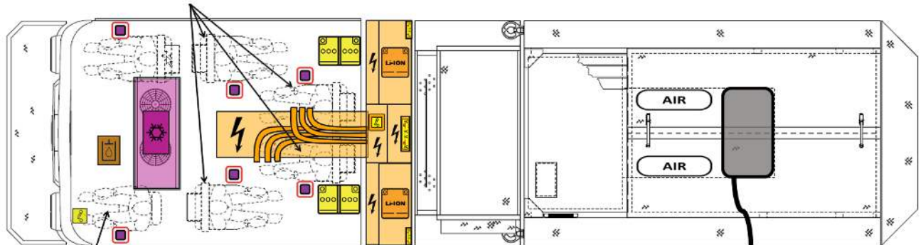
Optional Crew Cab Seat Locations
